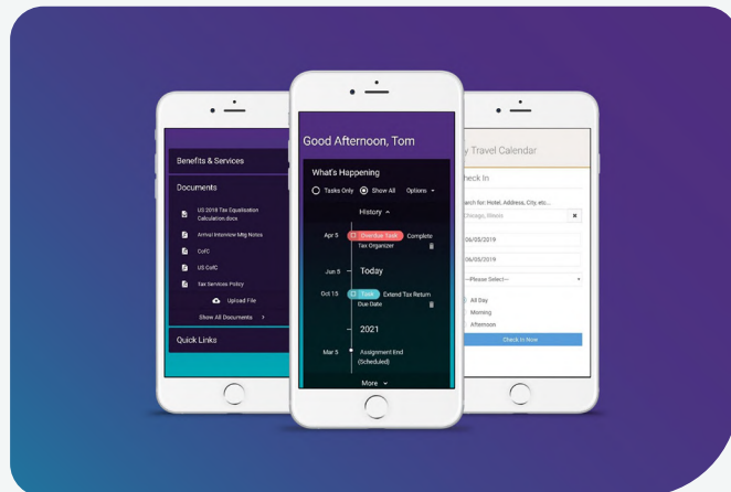
2: Mobile application
